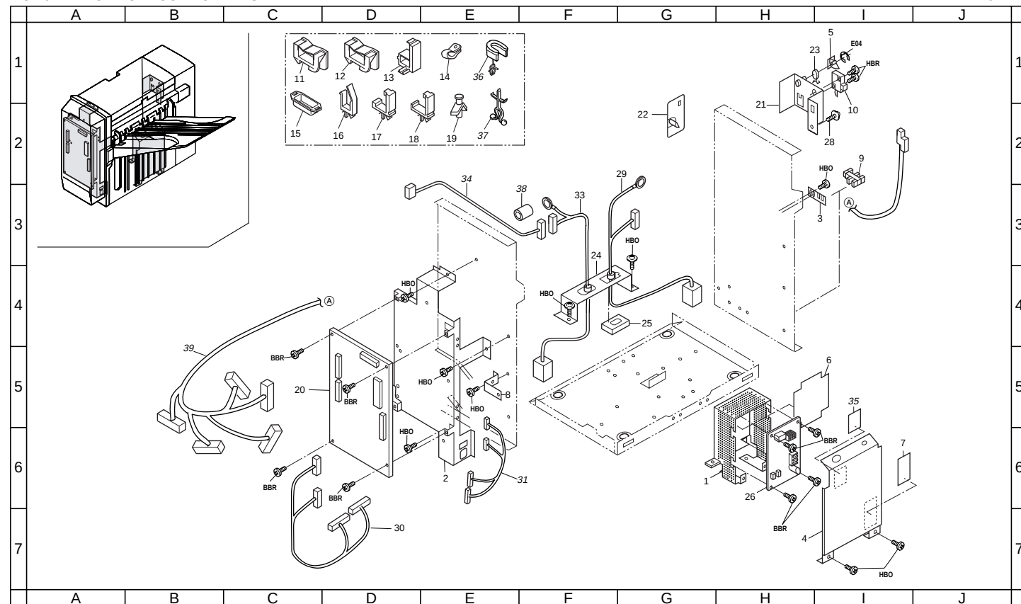
FIG. 6 ELECTRICAL COMPONENTS
