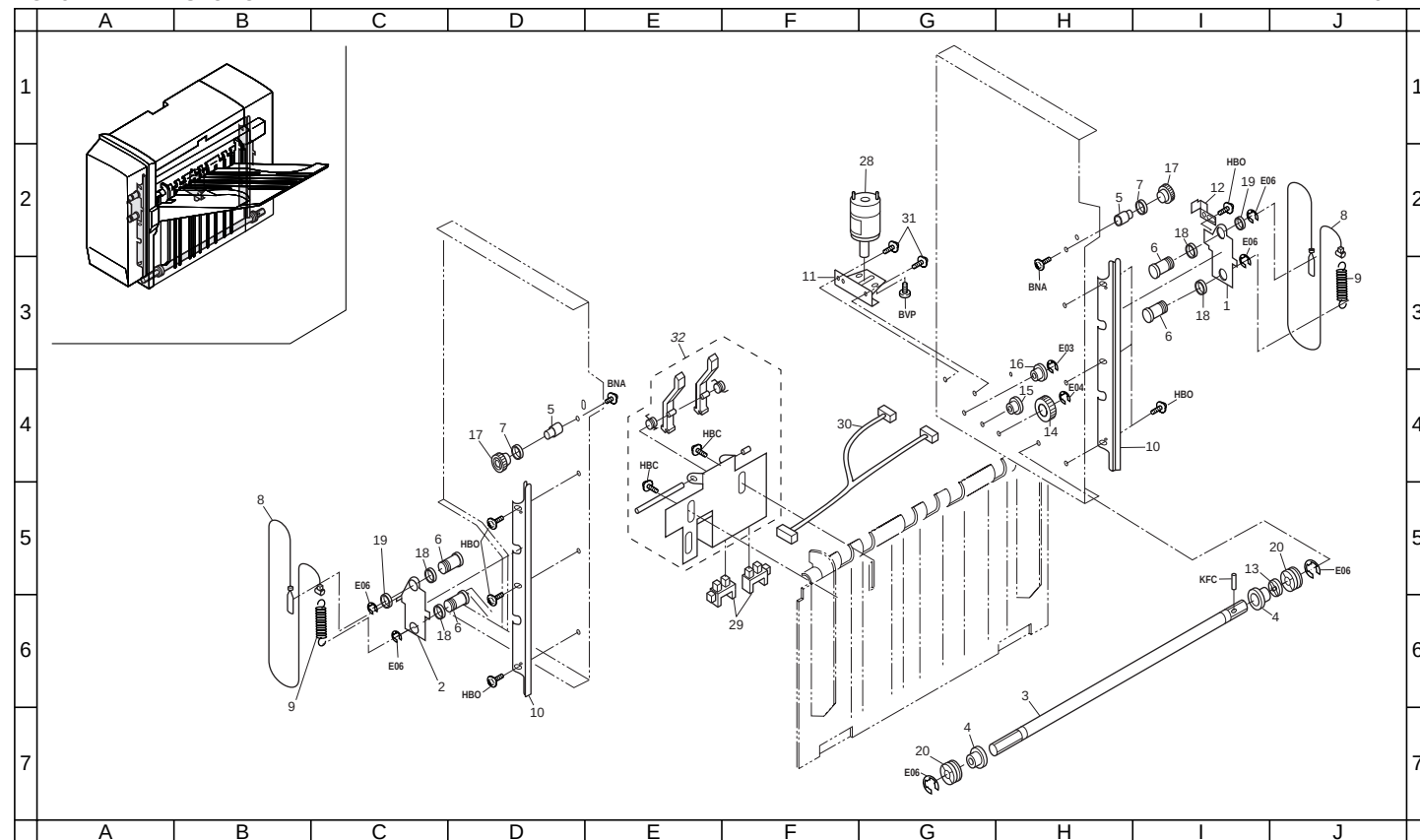
FIG. 5 ELEVATE SECTION
