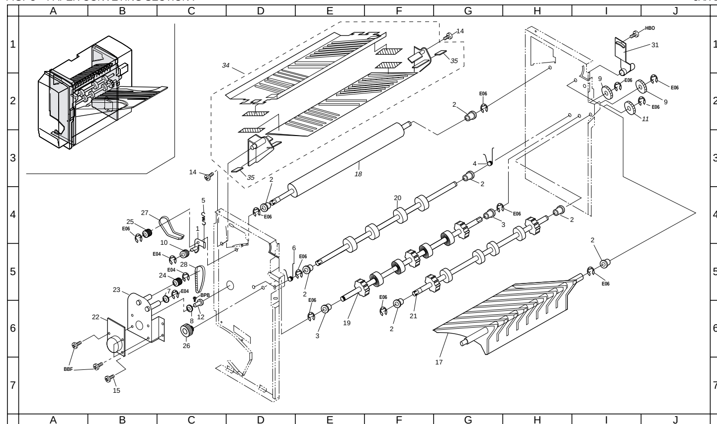
FIG. 3 PAPER CONVEYING SECTION I
