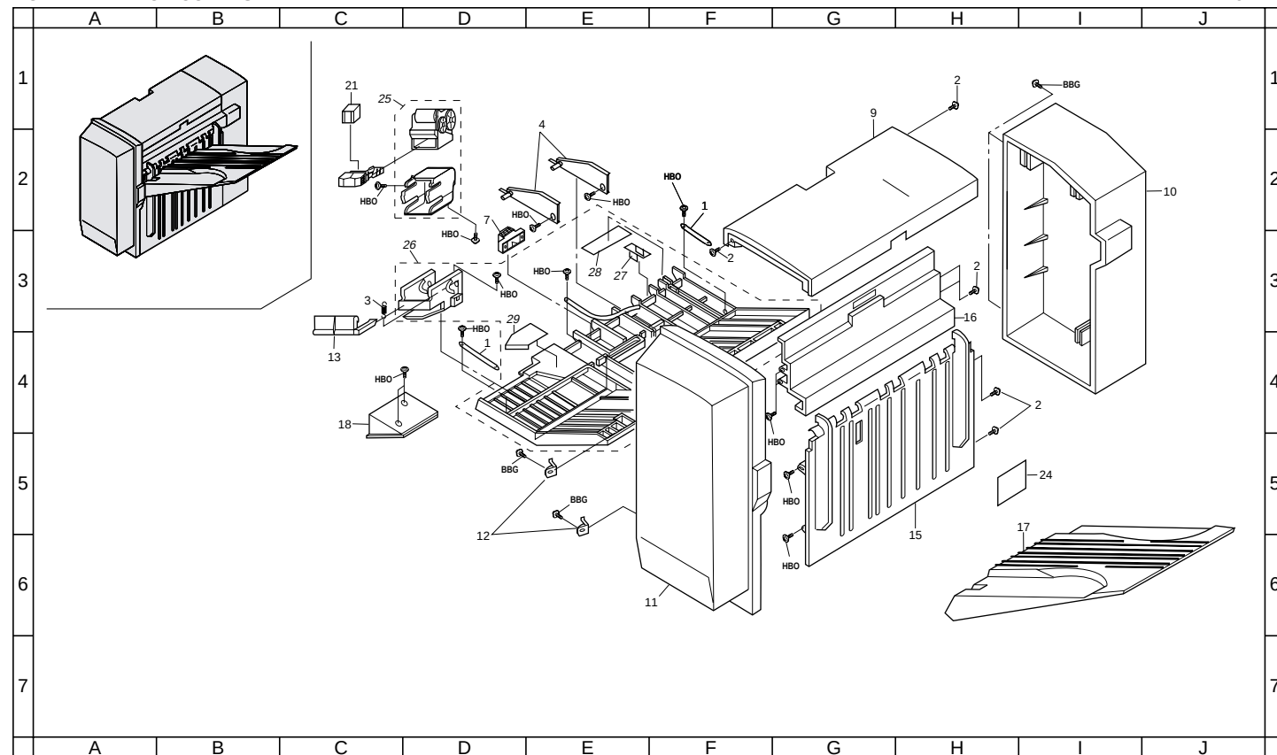
FIG. 1 EXTERIOR COVERS
